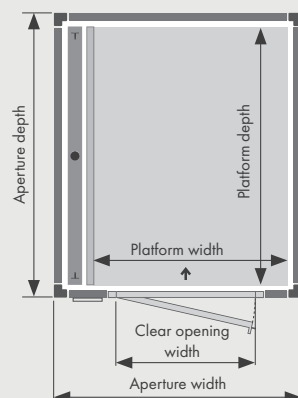
Aluminium structure
